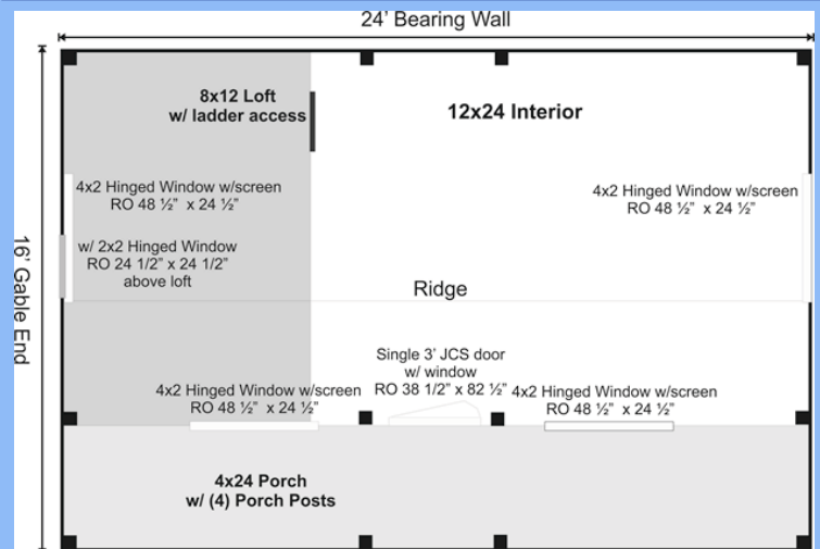
Option A Bearing Wall Porch
